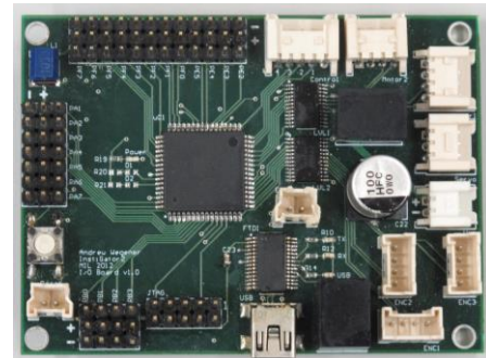
Figure 11: The I/O board.
